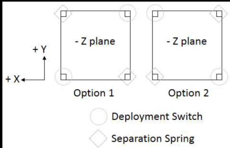
Figure 2-2. Separation Spring Placement Options.
