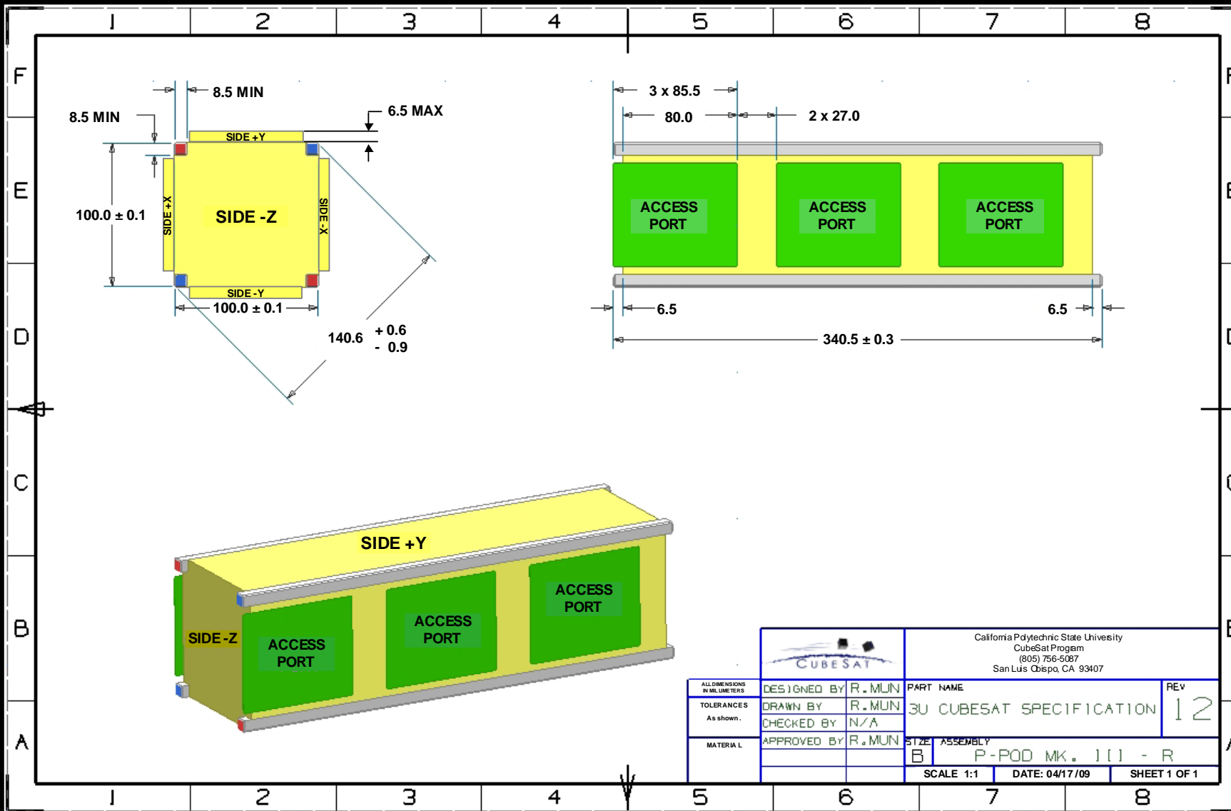
Figure 2-3. CubeSat Structure Specification Error! Reference source not found..
