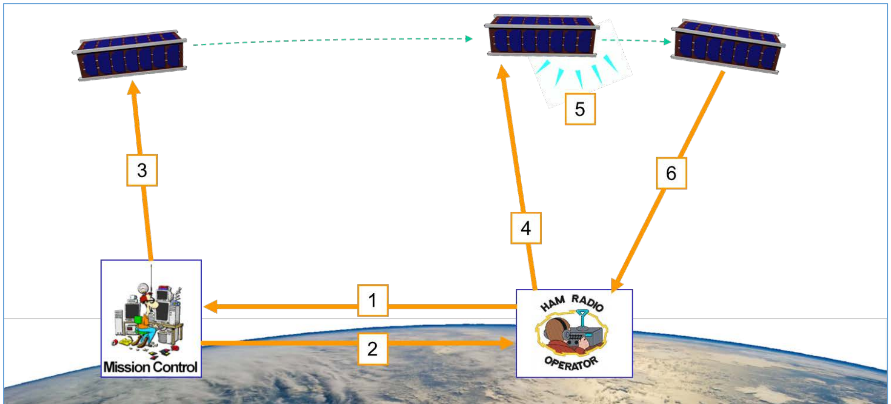
Figure 3-1. Selfie-Sat Concept of Operations.
